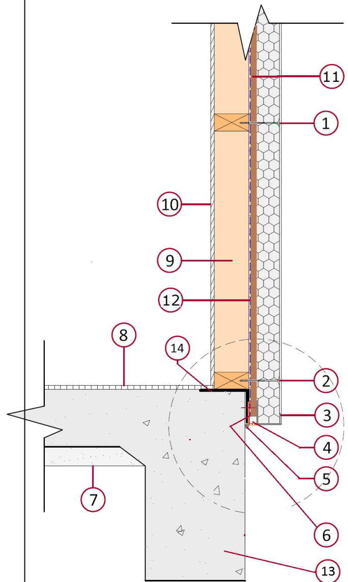
Fig 8C Panel Slab Edge Details-Cavity System
