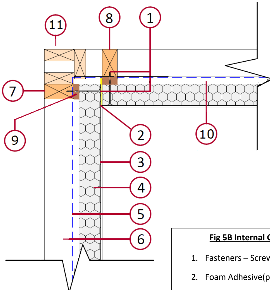
Figure 5B– INTERNAL CORNER - PLAN VIEW – Cavity System
