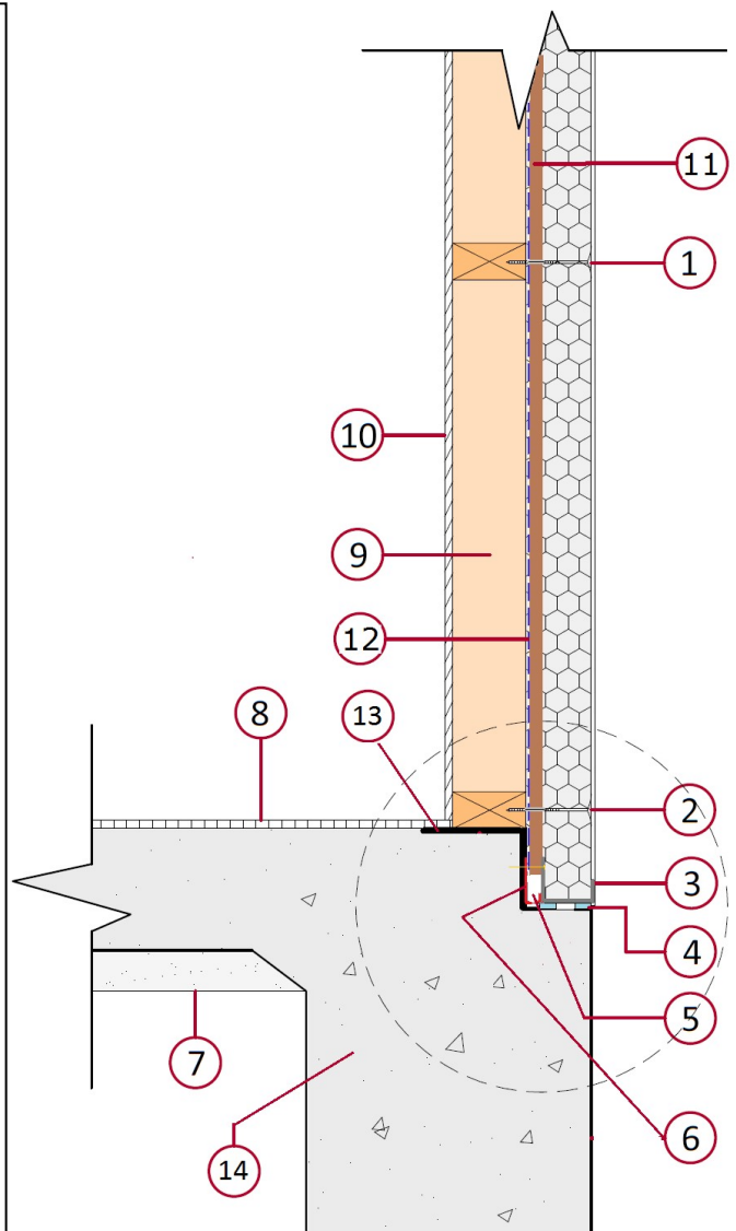
Fig 8B Panel Rebate Slab Details-Cavity System
