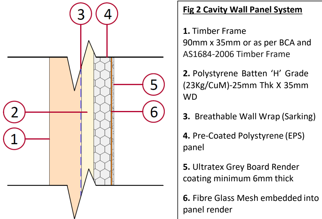
Sectional view for Ultratex Grey Board EIFS Cavity Wall Panel System
